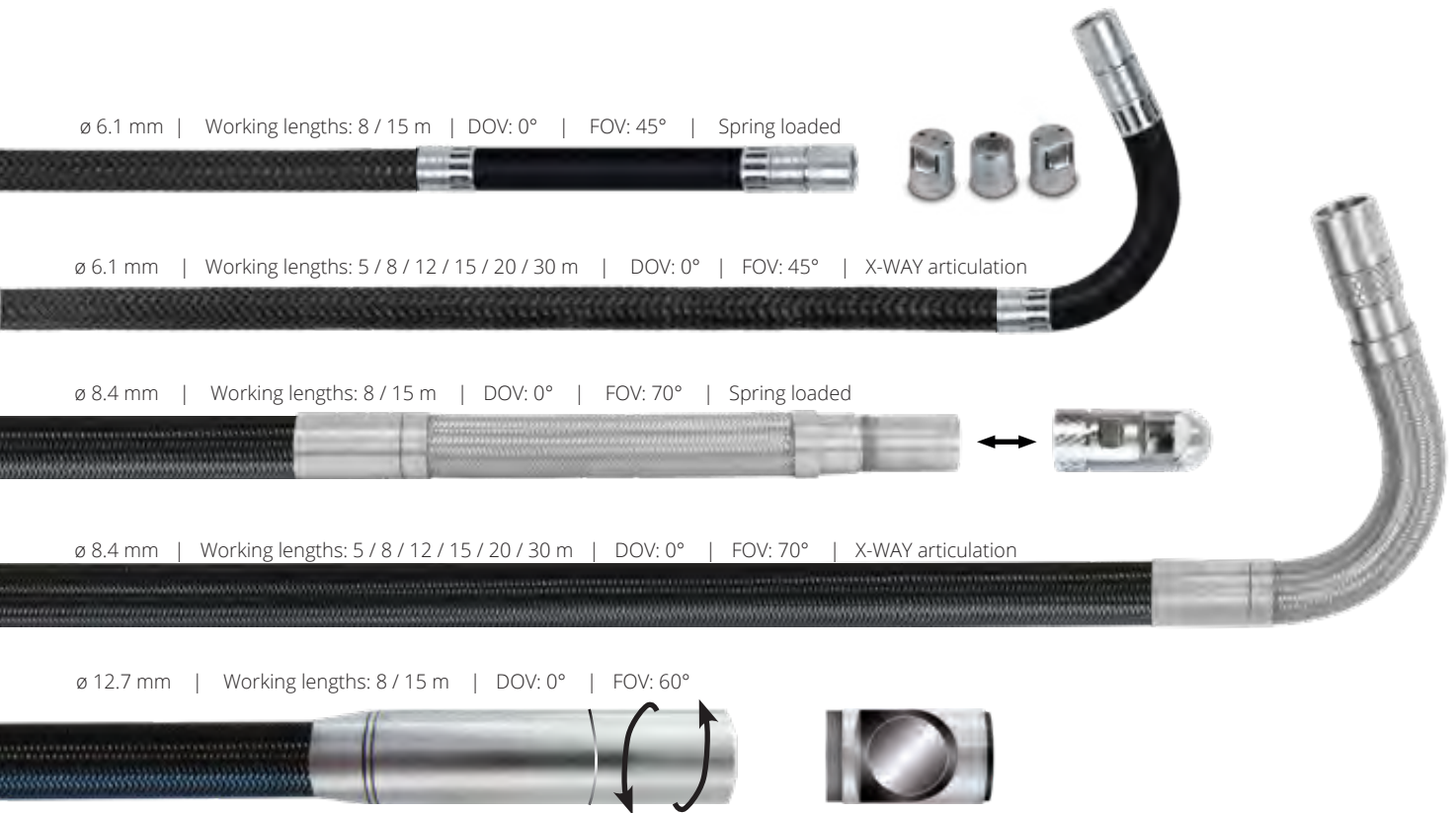
Continuously rotating head with side view adapter and variable rotation speed
