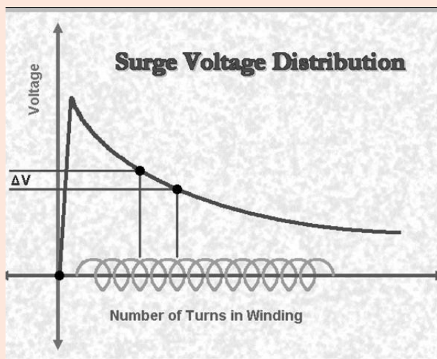
Figure 1: Initial impulse voltage distribution in a coil
