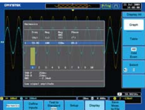
Harmonics
