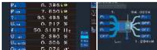
P4: DC power (panel output) P123: 3-phase power (power conditioner output) Urf4: Ripple rate \eta 1: Conversion efficiency f1: Frequency Uthd1: Voltage total harmonic distortion Uunb123: Unbalance rate Qfnd123: Fundamental wave reactive power
